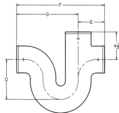
RUNNING TRAP w/4" SINGLE VENT
