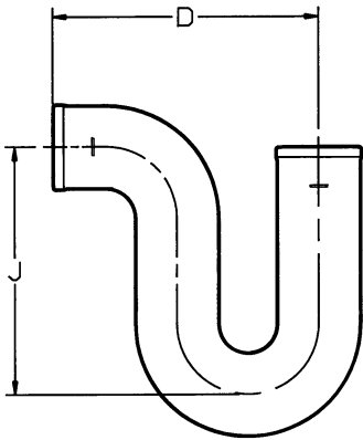
DEEP SEAL P-TRAP
