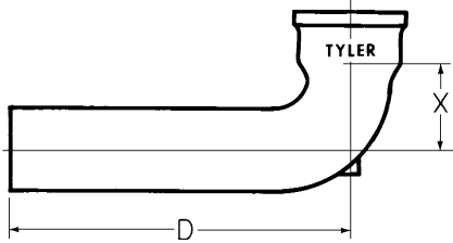
LONG QUARTER BEND
