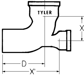
QUARTER BEND w/ Low Heel Inlet
