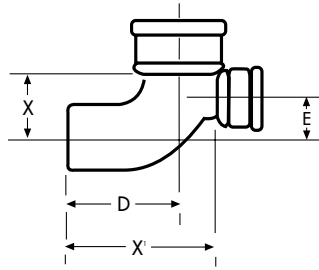
QUARTER BEND w/HIGH HEEL INLET
