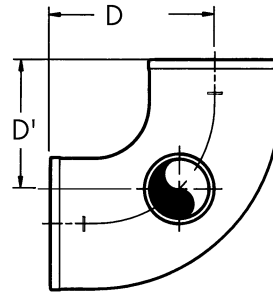
QUARTER BEND w/ 2" Side Opening
