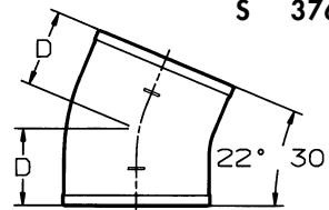
SIXTEENTH BEND
