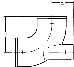
QUARTER BEND w/ 2" Heel Opening
