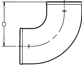
QUARTER BEND
