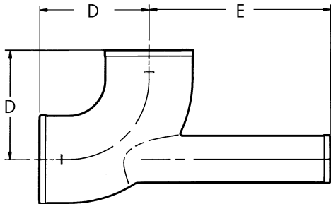
QUARTER BEND EXTENDED HEEL OPENING
