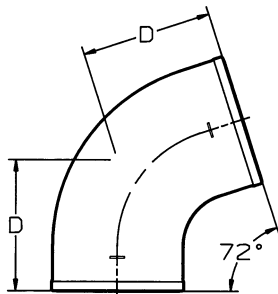
FIFTH BEND
