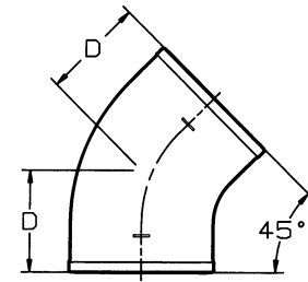
EIGHTH BEND
