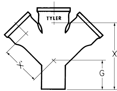
DOUBLE WYE
