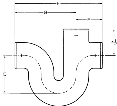
RUNNING TRAP w/4" SINGLE VENT
