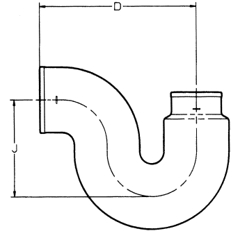
REDUCING P-TRAP
