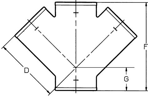
DOUBLE WYE
