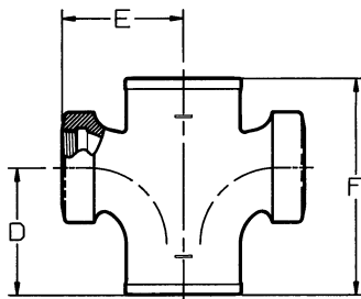
SAN TAP CROSS (No Baffle)
