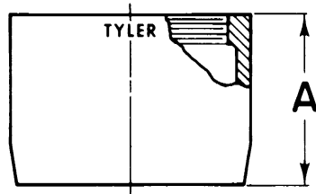
2-11 STANDARD FERRULE (Less Plug)
