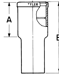
INSERTABLE JOINT (SV Only)
