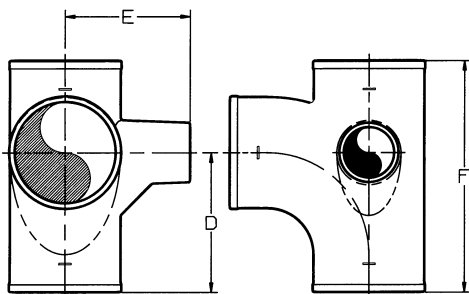
SAN TEE (w/2" 90° Side Opening on Center)
