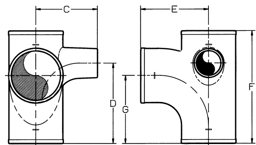
SAN TEE (w/2" 90° Side Opening Above Center) New Orleans Code
