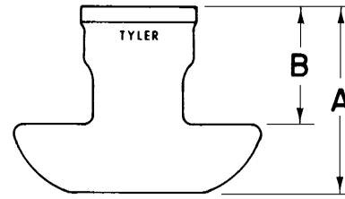
2-105 SEWER SADDLE
