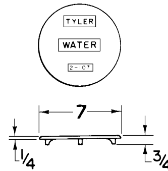
2-107 DROP LID Fits 6" Spigot
