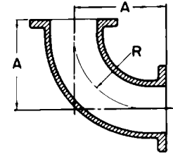
*90° Long Radius Bend (1/4)
